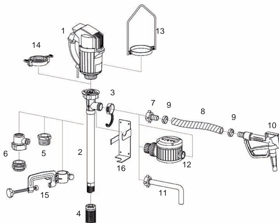
Fig. 1: Layout of pump (with components), non-explosion-proof
