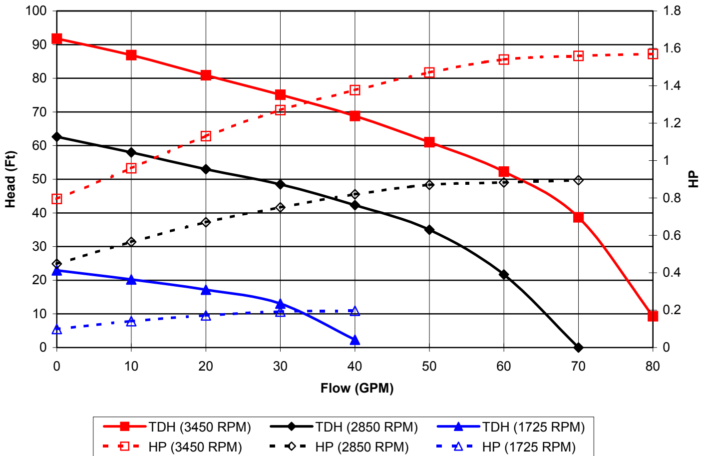
CRP Closed Impeller #4 (Based on Water @ Ambient Temp.)
