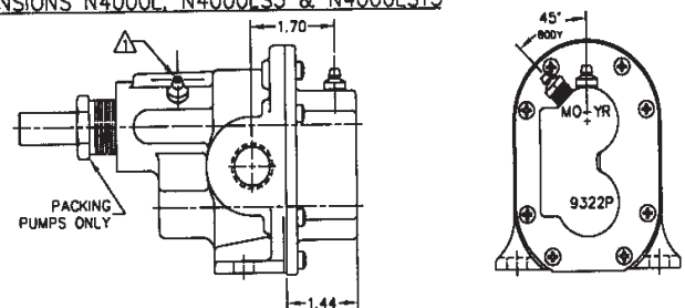
DIMENSIONS N4000L, N4000LS3 & N4000LS15
