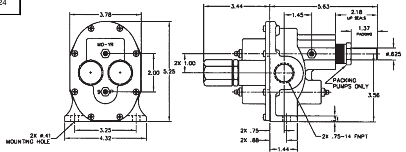
DIMENSIONS N7000L, N7000LS3 & N7000LS15
