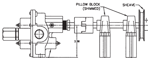
STANDARD N7000L(R) SERIES PUMP FIGURE 2
