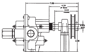
OPTIONAL N7000L(R)-02 SERIES PUMP (LONG DRIVE SHAFT) FIGURE 1
