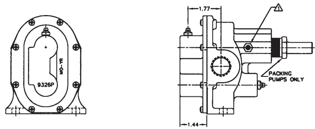
DIMENSIONS N7000L, N7000LS3 & N7000LS15
