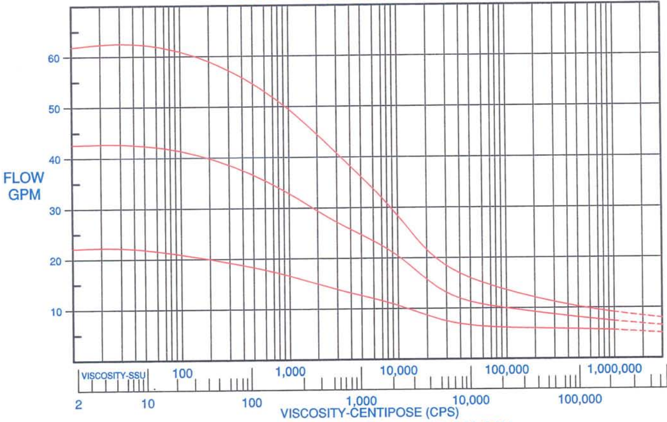
RB1420 2" PORTS .12 GAL/REV
